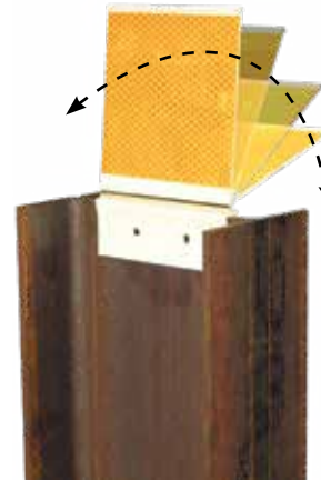
The I-Flex Strong Post with Urethane Hinge
