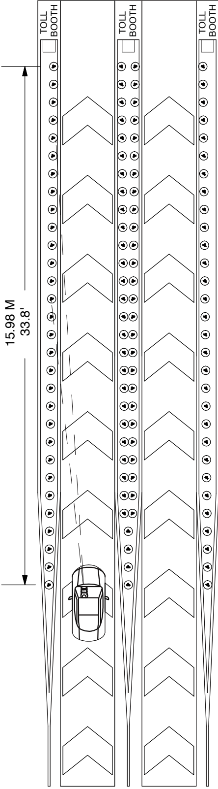
SET OF THIRTY POSTS - LAYOUT
