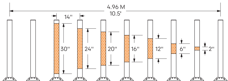
SET OF TEN POSTS — Layout Pattern
